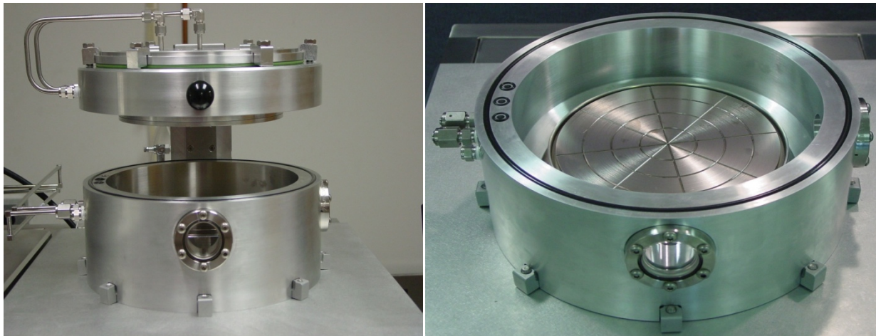
RIE Chamber
